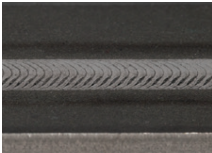
Plasma welding of titanium
